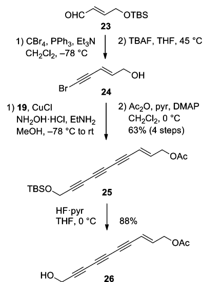
Scheme 9. Synthesis of 26
