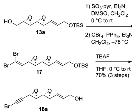
Scheme 4. Synthesis of 18a
