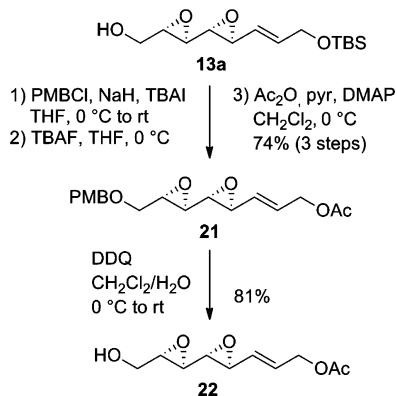
Scheme 8. Synthesis of 22
